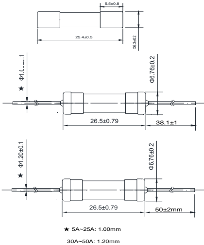
Dimensions (unit: mm)
