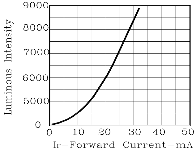
Luminous Intensity VS. Forward Current (Mcd)
