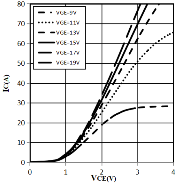
Fig 5. Typical output characteristic (T j =25°C)
