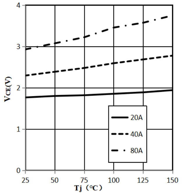
Fig 8. Typical collector-emitter saturation voltage as a function of junction temperature (V GE =15V)
