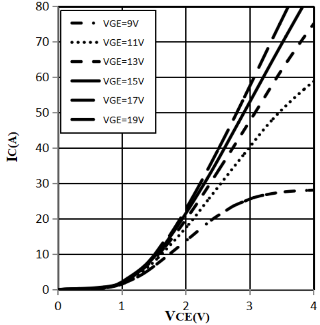
Fig 6. Typical output characteristic (T j =125°C)
