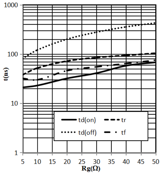
Fig 14. Typical switch time as a function of R_G (inductive load, T_J=25^\circ\text{C} , V_{CE}=400\text{V} , V_{GE}=15\text{V} , I_C=40\text{A} )
