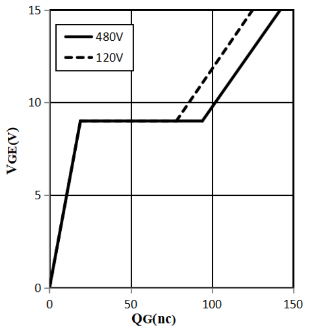
Fig 16. Typical gate charge ( I_C=40\text{A} )
