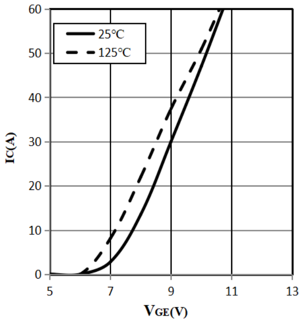
Fig 7. Typical transfer characteristic (V CE =20V)
