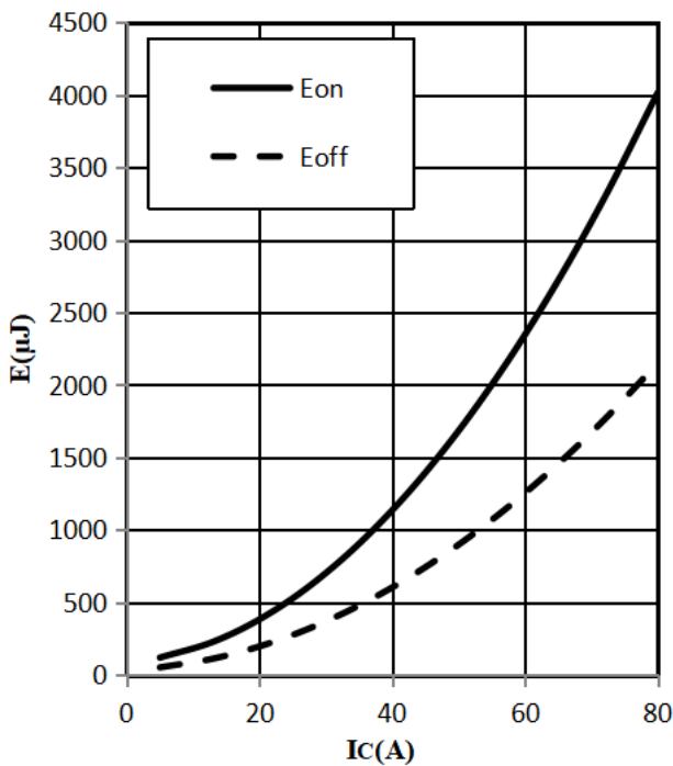
Fig 11. Typical switch energy as a function of I_C (inductive load, T_j=25^\circ\text{C} , V_{CE}=400\text{V} , V_{GE}=15\text{V} , R_G=10\Omega )
